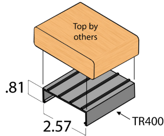
Add-A-Top TR400
